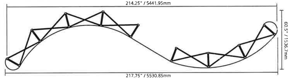
20' SERPENTINE
